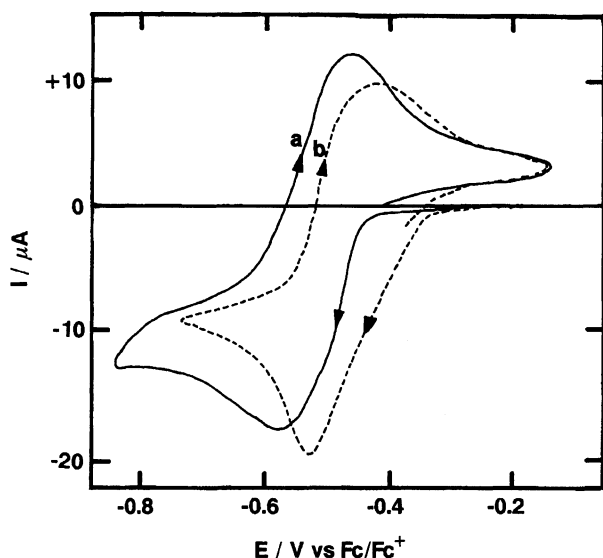
Fig. 2. Cyclic voltammograms of \text{NiI}_2(2,6\text{-Me}_2\text{C}_6\text{H}_3\text{NC})_2 ( 1a ) with and without excess 2,6- \text{Me}_2\text{C}_6\text{H}_3\text{NC} at Pt electrode in a 0.1 M \text{CH}_2\text{Cl}_2/\text{MeCN} (1:9)/ [\text{n-Bu}_4\text{N}][\text{ClO}_4] solution. (a): 1a (1.0 mM); (b): a mixture of 1a (1.0 mM) and 2,6-xylyl isocyanide (5.0 mM). Scan rate: 0.1 \text{ V s}^{-1} .
